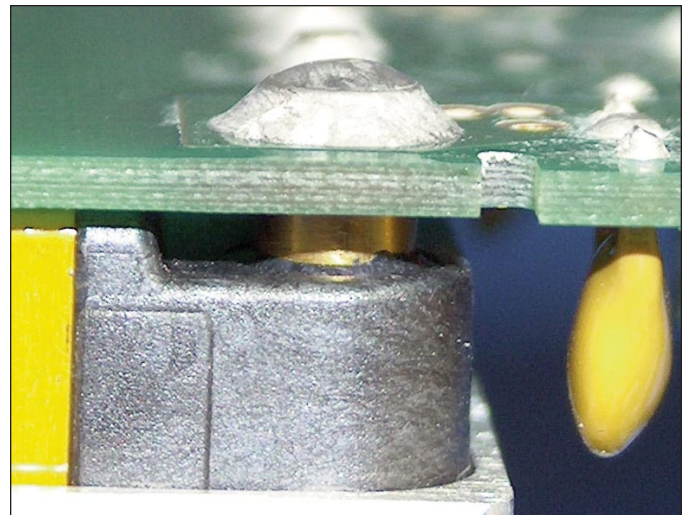
Figure 1 — Side profile of Maxi or Mini module's RoHS solder joint.
