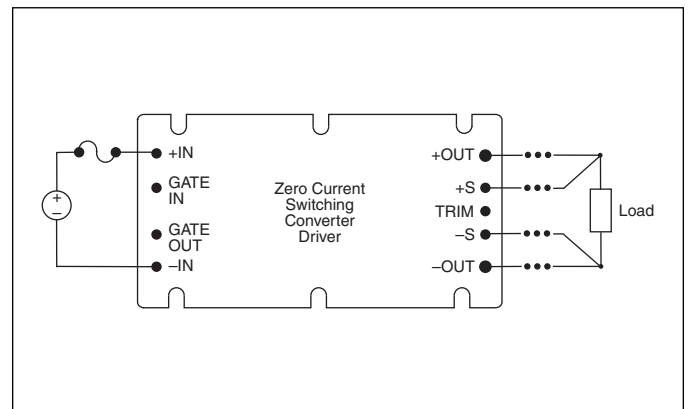
Figure 7–4 — Remote sensing
