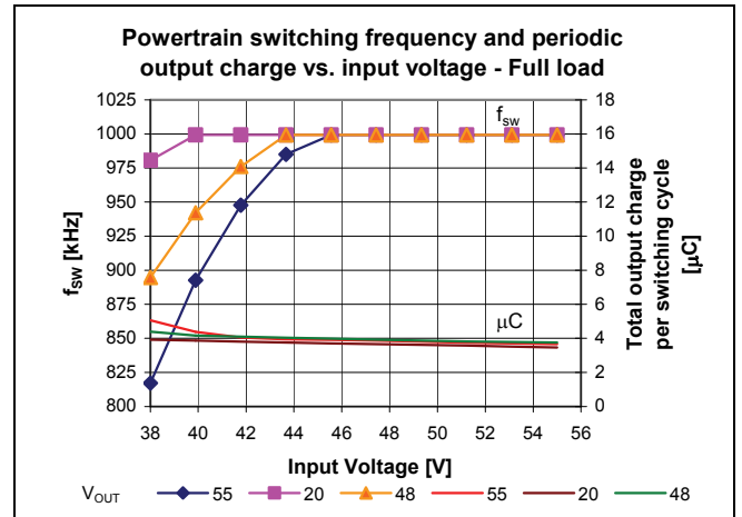
Figure 14 – Powertrain switching frequency and periodic output charge vs. V_{IN} , V_{OUT} ; I_{OUT}=4.17A
