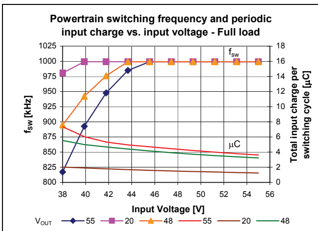
Figure 15 – Powertrain switching frequency and periodic input charge vs. V_{IN} , V_{OUT} ; I_{OUT}=4.17A
