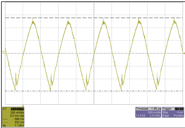
Figure 13 – Typical output voltage ripple waveform, T_{CASE}=30^{\circ}C , V_{IN}=45V , V_{OUT}=48V , I_{OUT}=4.17A , no external capacitance.
