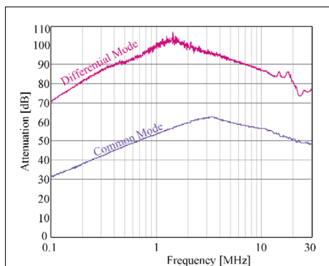
Figure 2 – Typical attenuation; QPI-8 network analyzer attenuation curves.
