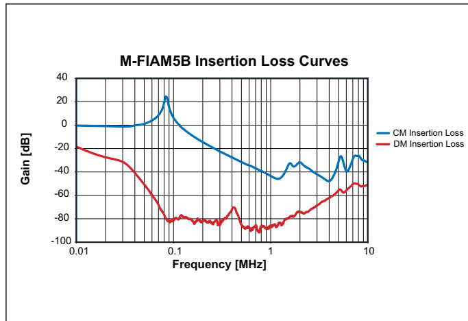
Figure 5 — Insertion Loss
