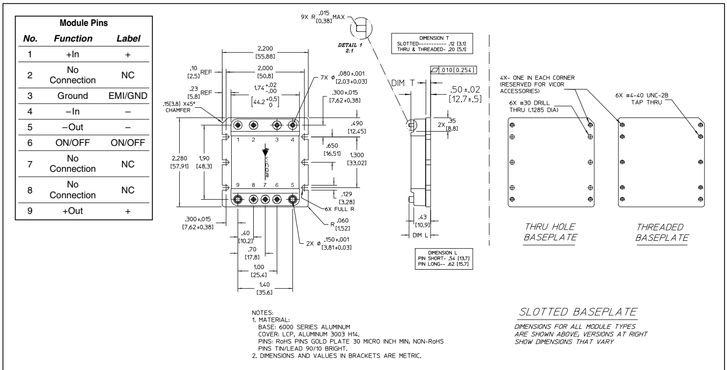
Figure 8 — Mechanical diagram
