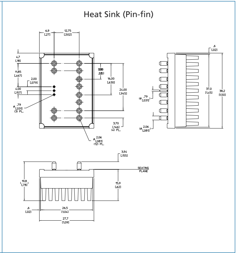
Figure 19 — Pin-fin heat sink outline
