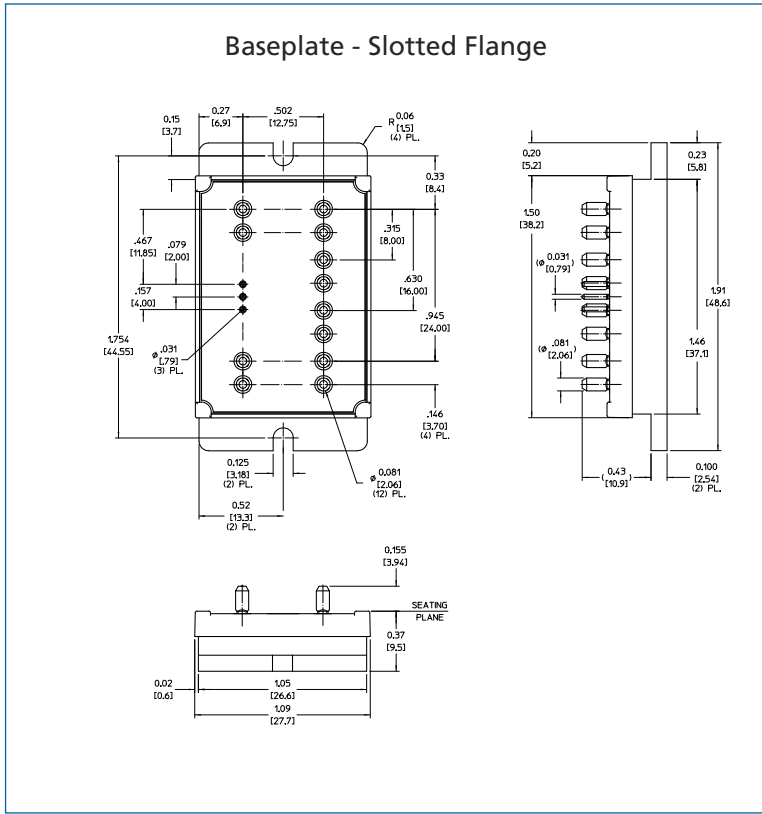
Figure 18 — Module outline
