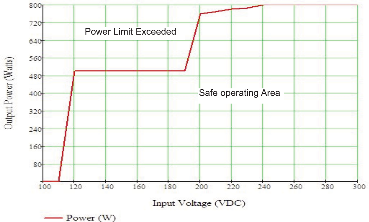
PFC Micro Output Power vs. DC Input Voltage
