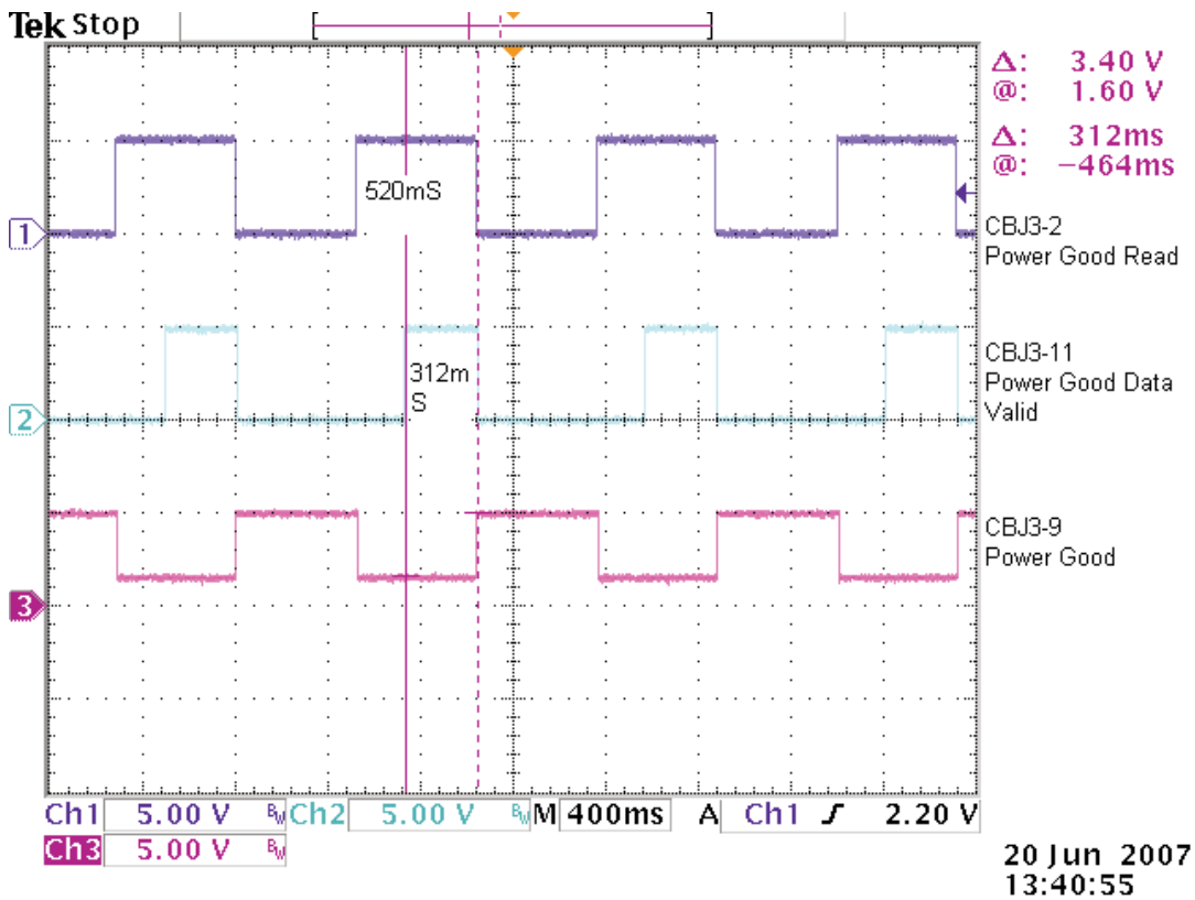
PowerGood Read with Defective Module
