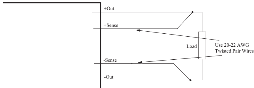
Figure 5. Remote Sense
