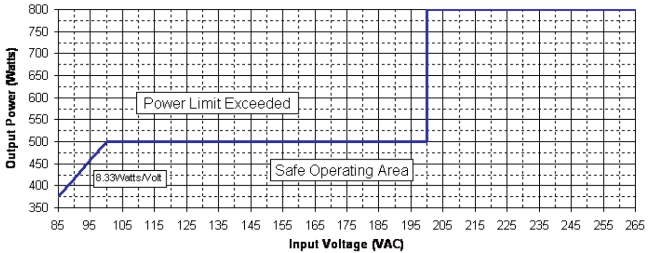
PFC Micro Output Power vs. AC Input Voltage
