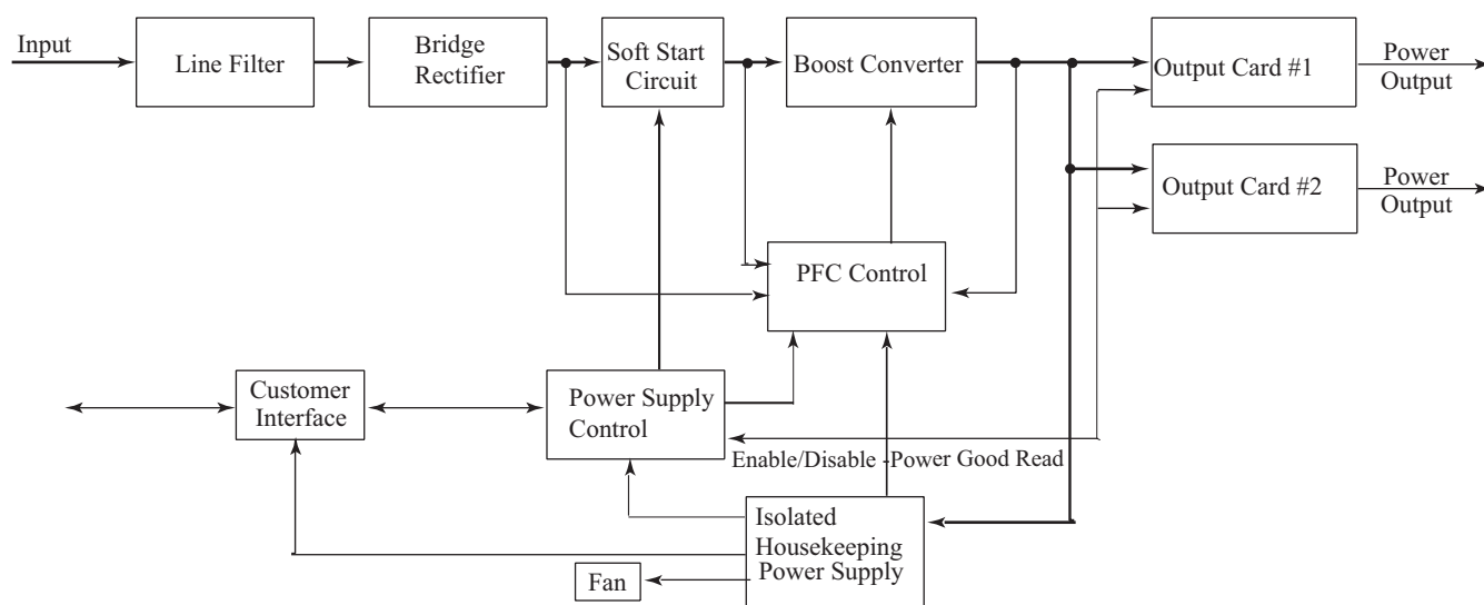
Figure 1. PFC Micro Architecture
