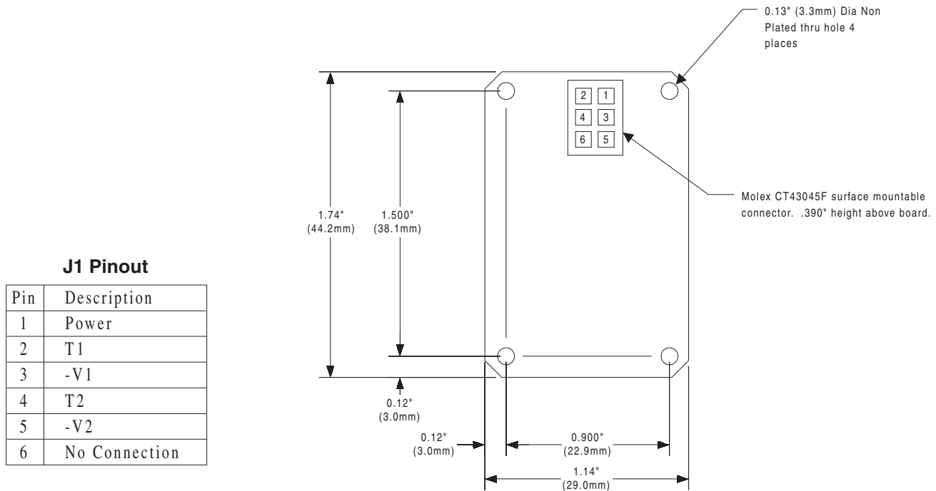
Figure 2. Mechanical Drawing
