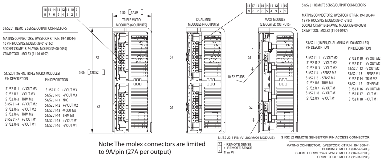
Figure 3. Output Power Connections
