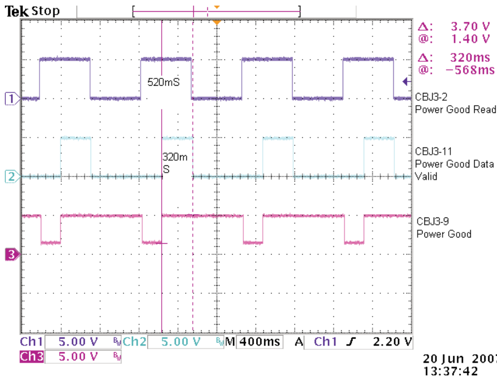
PowerGood Read with Good Module
