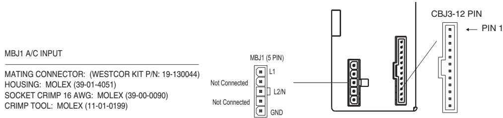
Figure 2. Input Power Terminal MBJ1
