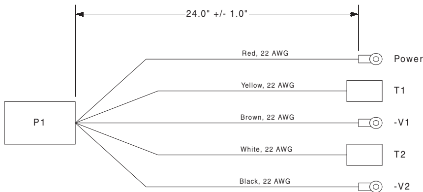
Figure 3. Cable Drawing
